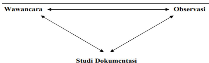
Gambar 1. Alur Penelitian
